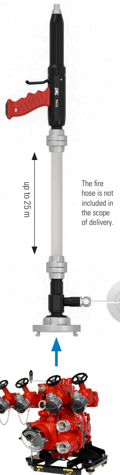
AWG SANISTREET FLEX can be used with any pump that provides 60 l/min at 7.5 bar.
